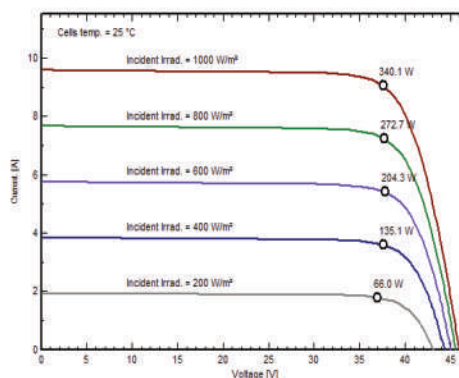
I-V Curve of 340W at 25°C cell temp. and different Irradiance level
